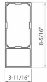
Beam cross-section
